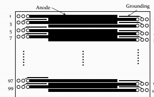
(B) The design of the printed circuit board (PCB)
