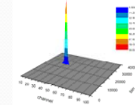
(B) MALDI-TOF spectrum of Angiotensin II (DRVYIHPF, m/z=1046.5) after the detector was charged up with matrix ions and peptide ions for 2 hrs
